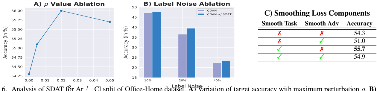
Figure 6. Analysis of SDAT for Ar/Cl split of Office-Home dataset. A) Variation of target accuracy with maximum perturbation \rho . B) Comparison of accuracy of SDAT with DAT for different ratio of label noise. C) Comparison of accuracy when smoothing is applied to various loss components.
